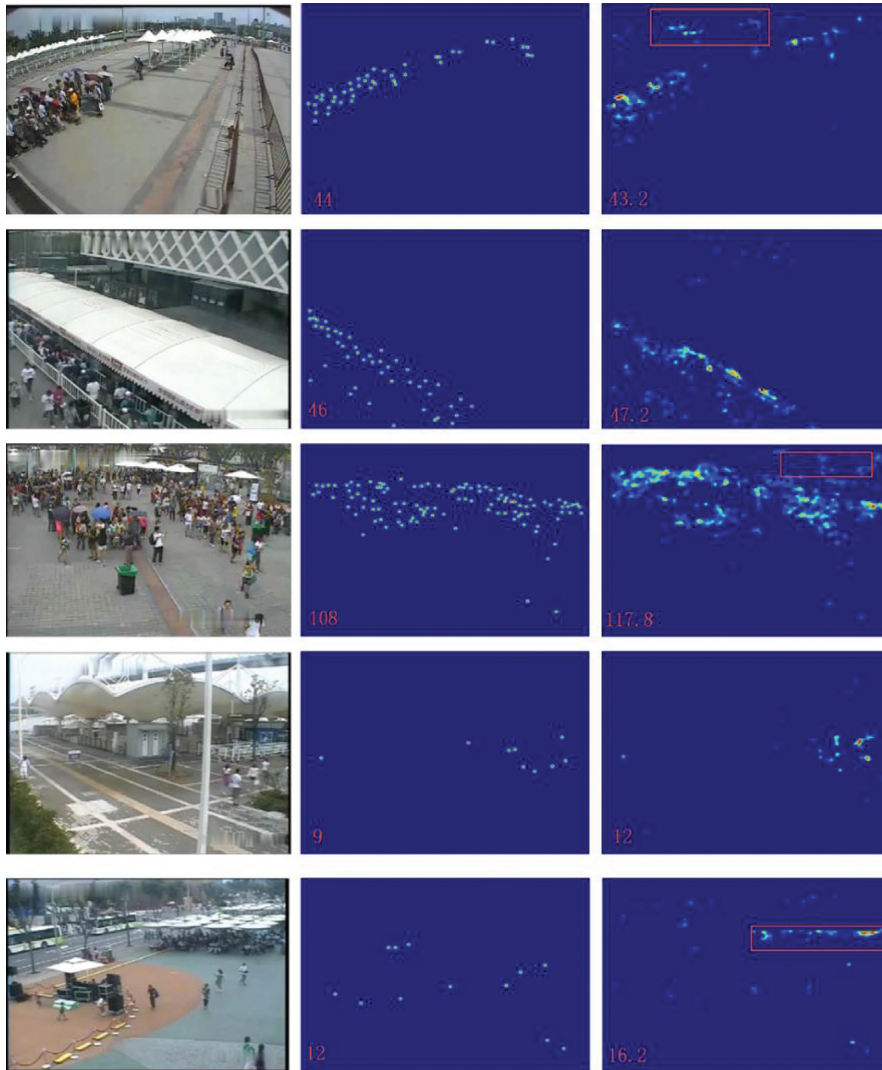
FIGURE 8: Comparison of visual results on WorldExpo'10. The first, second, and third columns show test samples, the corresponding ground truth, and the generated density map, respectively. The box outlined in red represents the area where we mistook the background for a head.
