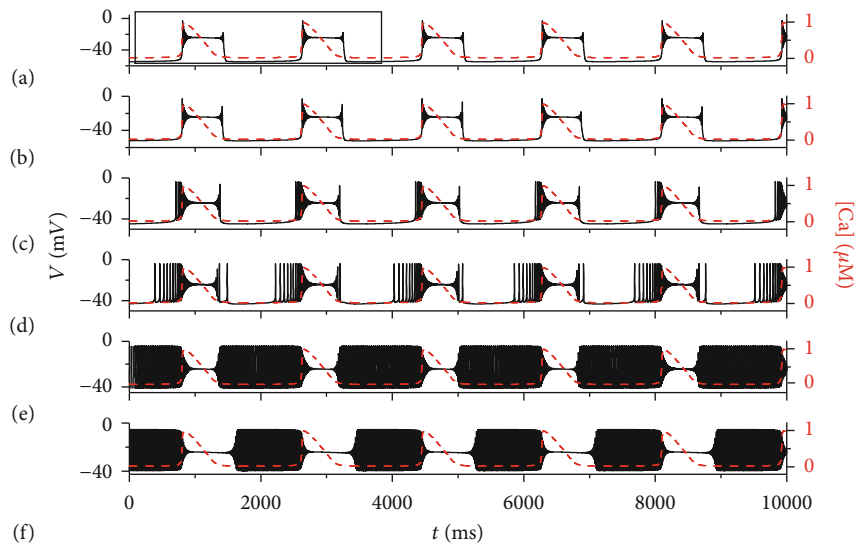
FIGURE 3: The full system (1a)–(3b) exhibits different firing patterns under different electric currents at k_1 = 0.1 , k_2 = 3 \text{ s}^{-1} , \alpha = 1 \text{ M}\Omega^{-1} , \beta = 0.00006 \text{ M}\Omega^{-1} \cdot \text{V}^{-2} \cdot \text{s}^{-2} . The red dashed line represents the time course of intracellular calcium concentration [Ca] . (a) I_{extz} = -2 \mu A/cm^2 ; (b) I_{extz} = 5 \mu A/cm^2 ; (c) I_{extz} = 25 \mu A/cm^2 ; (d) I_{extz} = 30 \mu A/cm^2 ; (e) I_{extz} = 40 \mu A/cm^2 ; (f) I_{extz} = 50 \mu A/cm^2 .
